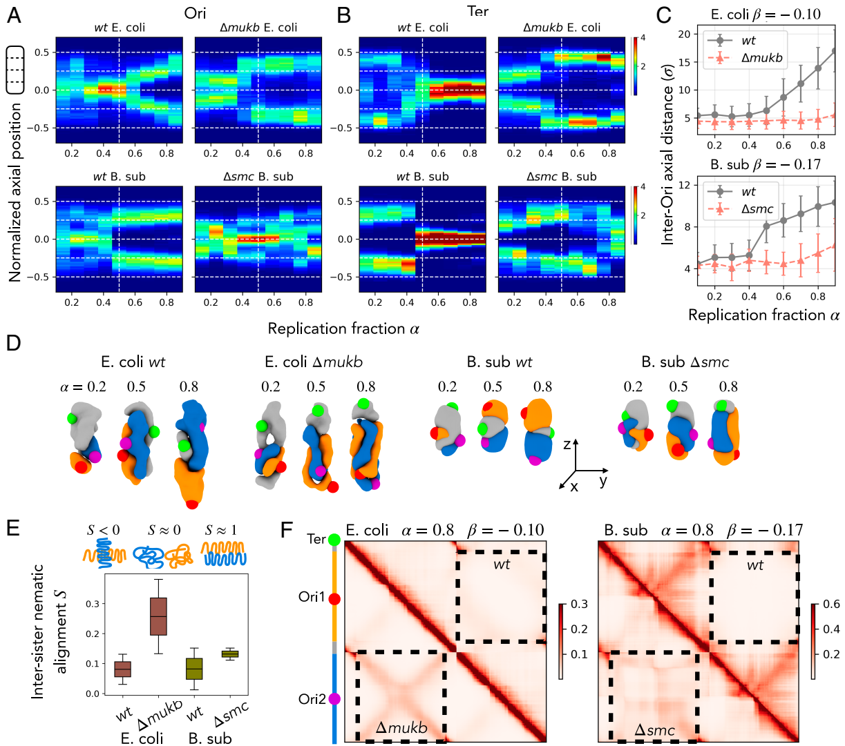
Fig. 3. Structural transitions, segregation dynamics, and intersister interactions during replication. Kymographs showing the cell cycle axial dynamics of (A) the two ori and (B) ter across replication fractions \alpha for E. coli (Top) and B. subtilis (Bottom). The corresponding mutants SMC-deficient E. coli and B. subtilis are shown in adjacent subpanels. The white horizontal lines denote the nucleoid quarters and the vertical white line denotes mid-replication. wt chromosomes undergo a mid-replication transition in which the ter moves toward the nucleoid center and the two ori separate toward opposite poles, whereas mutants lacking SMCs fail to undergo this rearrangement. (C) Inter-ori axial distance as a function of replication fraction, showing ori segregation in wt but proximal ori pair in \Delta mukb and \Delta smc mutants. (D) Representative 3D structures at early ( \alpha = 0.2 ), mid ( \alpha = 0.5 ), and late ( \alpha = 0.8 ) replication, illustrating wt ori splitting and ter repositioning versus persistent overlap and nematic alignment in mutants. Two ori and ter are red, purple, and green spheres, respectively. Chromosomes shown in density representation with two sisters in orange and blue, and unreplicated DNA in gray. (E) Intersister nematic alignment parameter S for \alpha = 0.8 , where S varies from -1/2 for perpendicular, to 0 for random isotropic, to 1 for perfectly aligned polymer. wt demonstrates more isotropic organization compared to SMC mutants with strong nematic alignment ( S > 0.2 ) of replicated arms. (F) Simulated sister-chromosome-resolved Hi-C maps at \alpha = 0.8 for E. coli and B. subtilis . The Upper triangle shows wt versus SMC mutants \Delta mukb and \Delta smc in the Lower triangles; intersister interaction blocks are highlighted by dashed rectangular boxes. SMC mutants show an increase in overall intersister contacts impeding segregation. The unsegregated state has nematic alignment that generates an X-shape in the intersister contact map. Together, these analyses show that SMC-mediated long-range compaction drives the structural transitions necessary for robust coreplication segregation.
